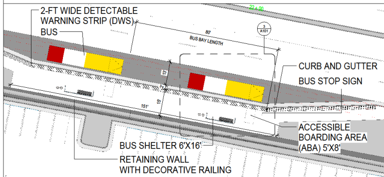
2 OPTION D - TYPICAL TANGENT BAY DIMENSIONS SCALE: 1"=15'
