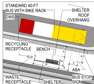
3 OPTION D - BUS SHELTER SCALE: 1/8"=1'-0"
