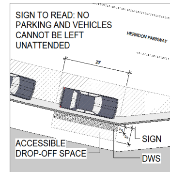
4 OPTION D - PASSENGER DROP-OFF SCALE: 1/8"=1'-0"
