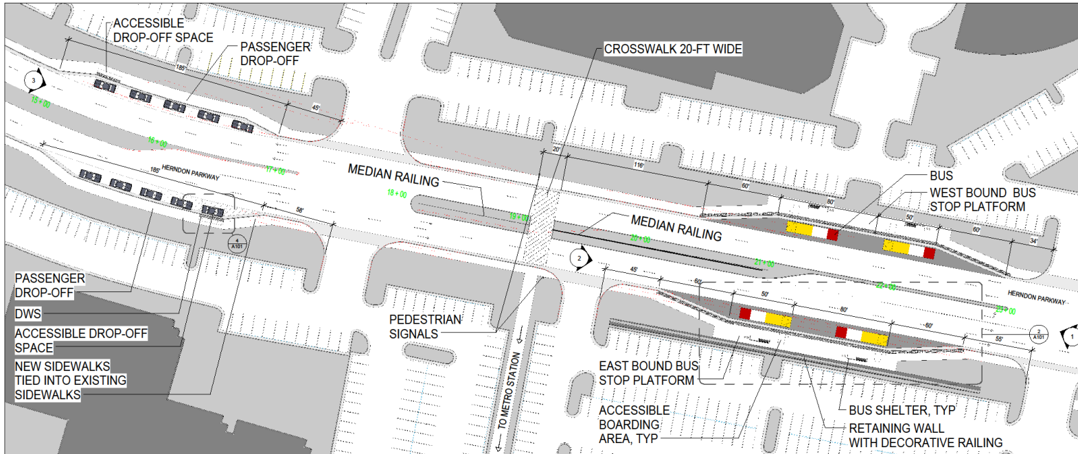
1 OPTION D - SITE PLAN SCALE: 1"=30'
